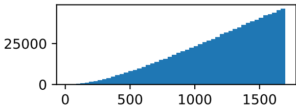
distance
